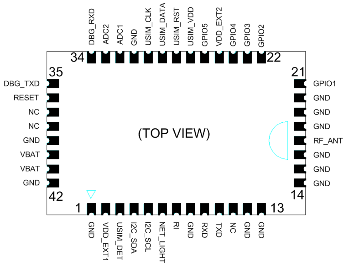
Figure.1 Pin Assignment
